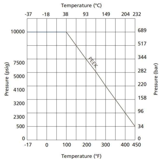
TBVH Series
