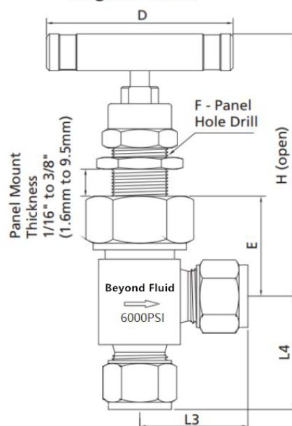
Angle Pattern
