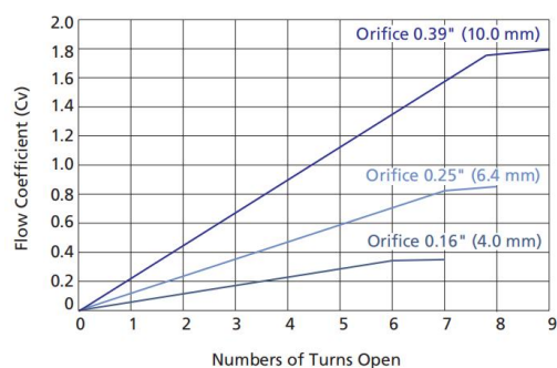
Regulating Stem
