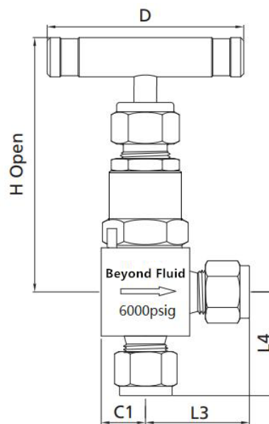
Angle Pattern
